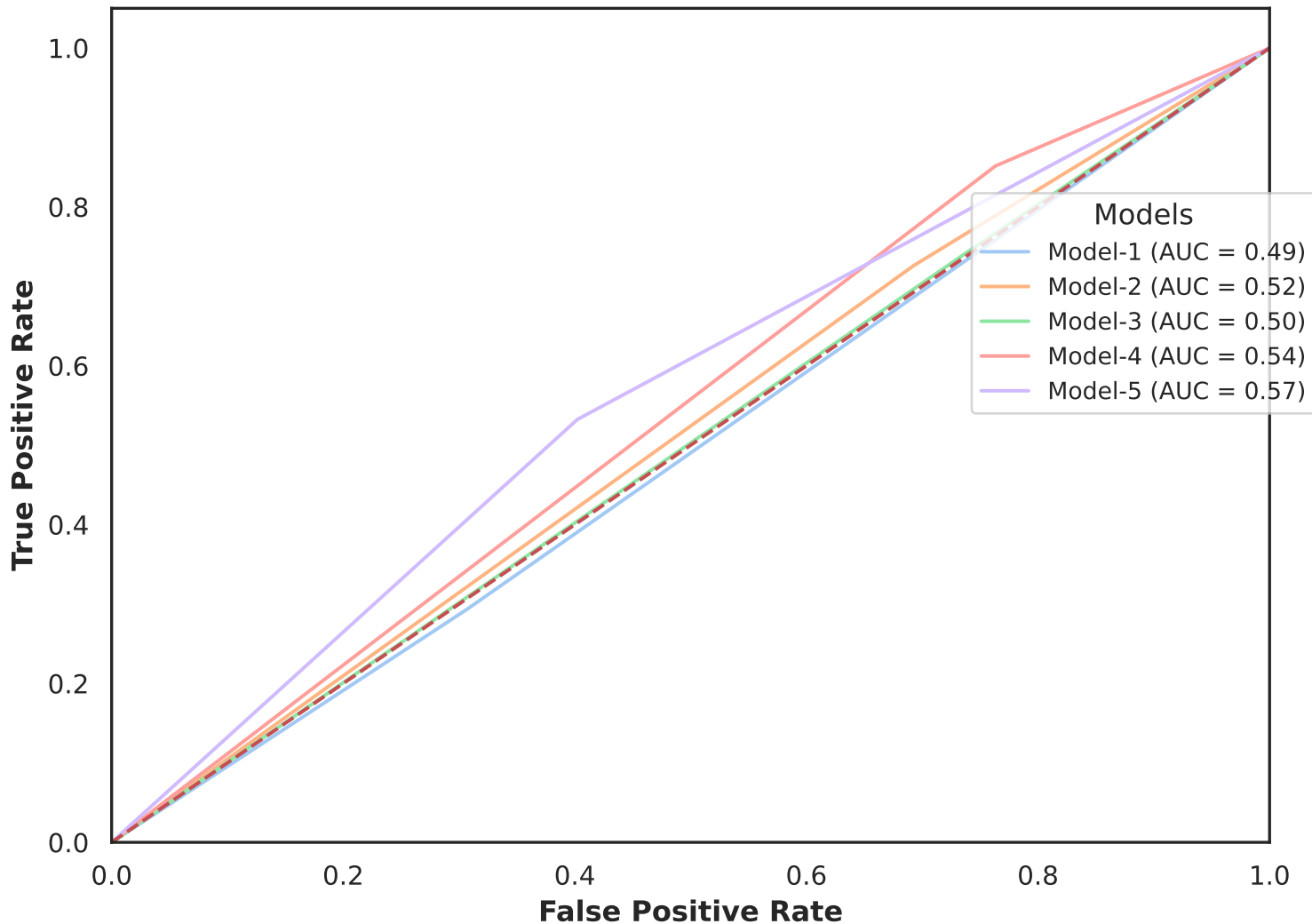
Combined ROC Curves for Adherence Score Across Models
